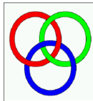
Figure 2. The classic Borromean rings.
