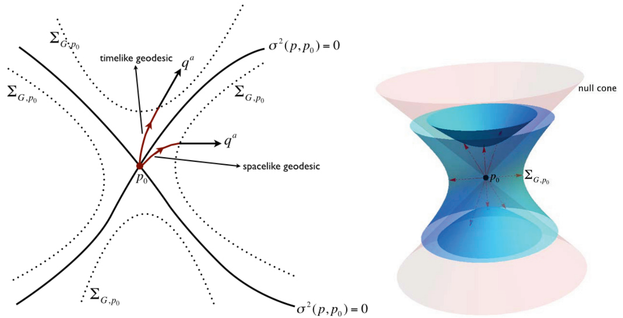
(a) Equi-geodesic surfaces \sigma_G attached to an event p_0 in an arbitrary curved spacetime.
